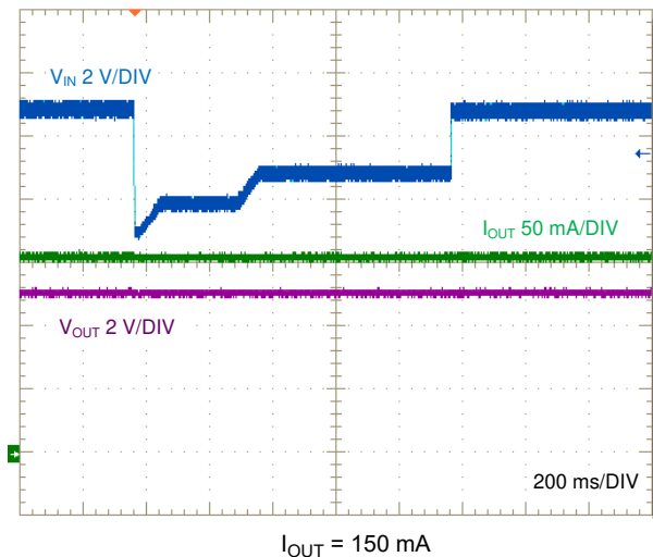
I_{OUT} = 150 mA Figure 8-13. Input Transient (Automotive Cold Crank Profile)
