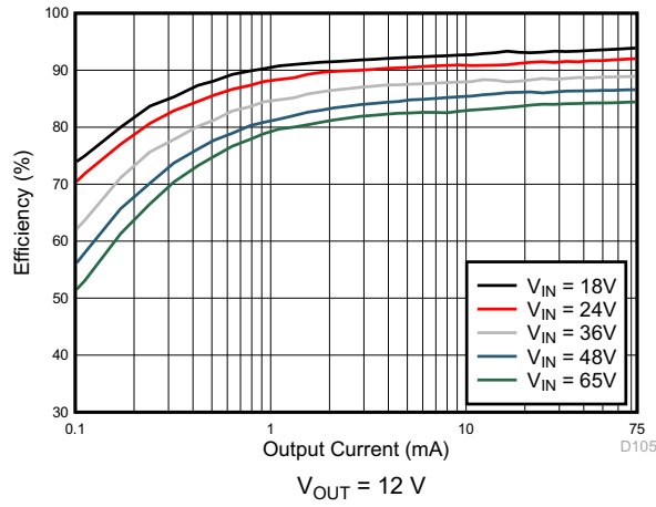
Figure 8-22. Efficiency
