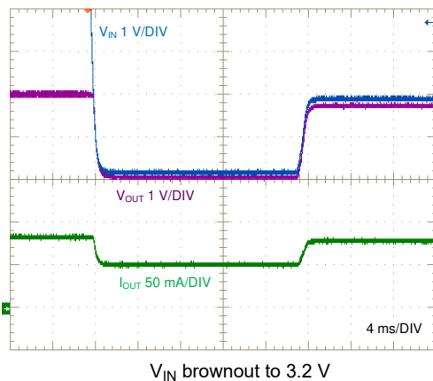
V_{IN} brownout to 3.2 V Figure 8-10. Dropout Performance, 75-mA Resistive Load
