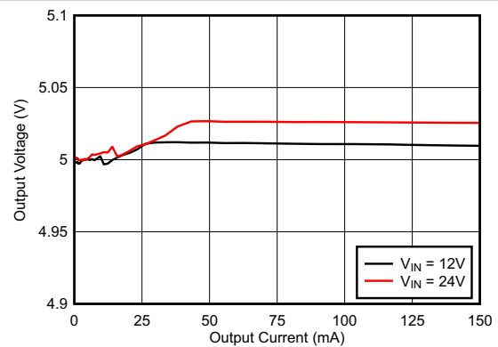
Figure 8-3. Load Regulation
