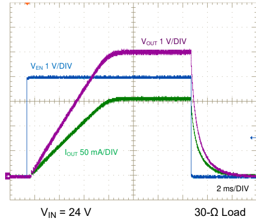
V_{IN} = 24 V 30- \Omega Load Figure 8-9. Enable ON and OFF
