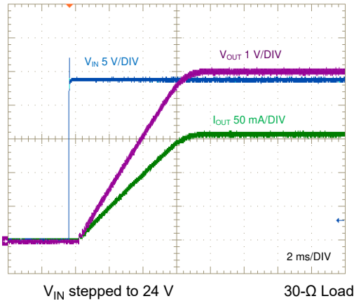
V_{IN} stepped to 24 V 30- \Omega Load Figure 8-8. Startup, Full Load
