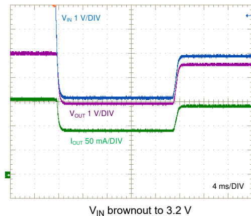
V_{IN} brownout to 3.2 V Figure 8-11. Dropout Performance, 150-mA Resistive Load
